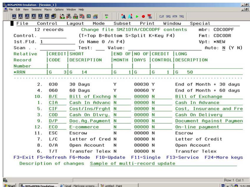
Sample Multi-Record Update Screen
